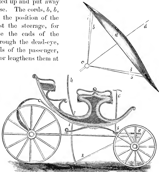
VINEY AND POCOCK'S CHARVOLANT.
